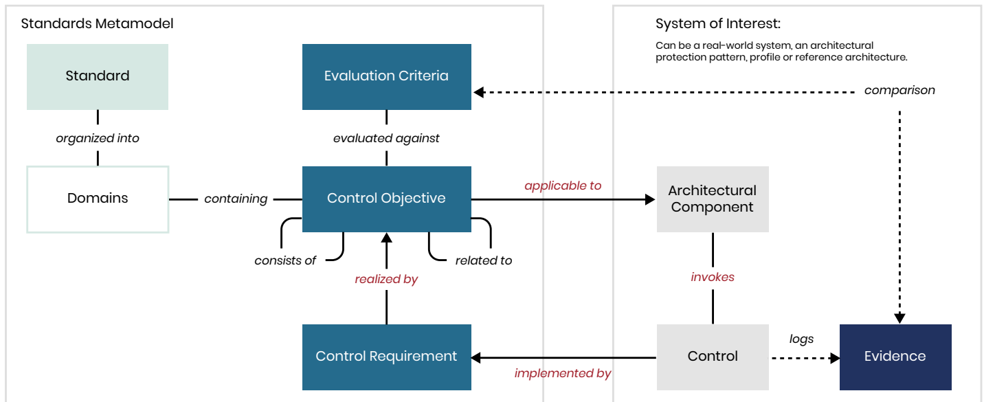
Figure 3. Compliance Metamodel
