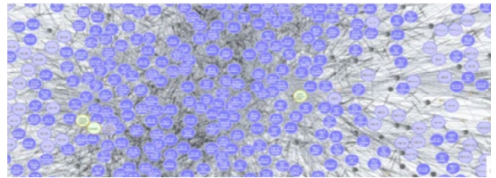
Figure 4. Multi-regulatory Compliance
