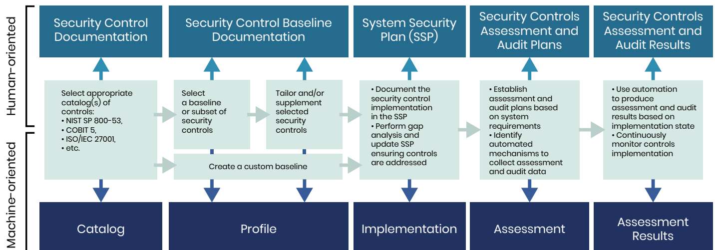
Figure 1. OSCAL Architecture
